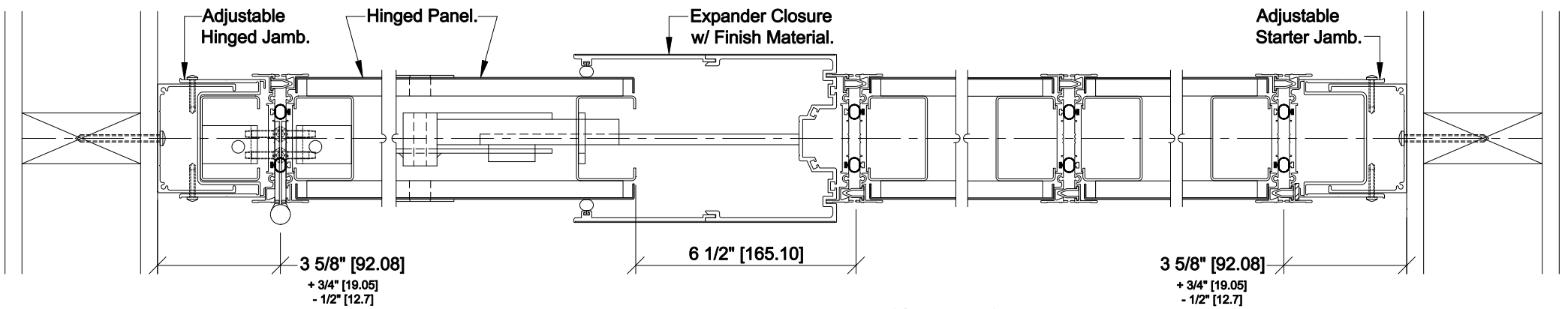
Horizontal Detail - Model 3020 (Cap-type)
