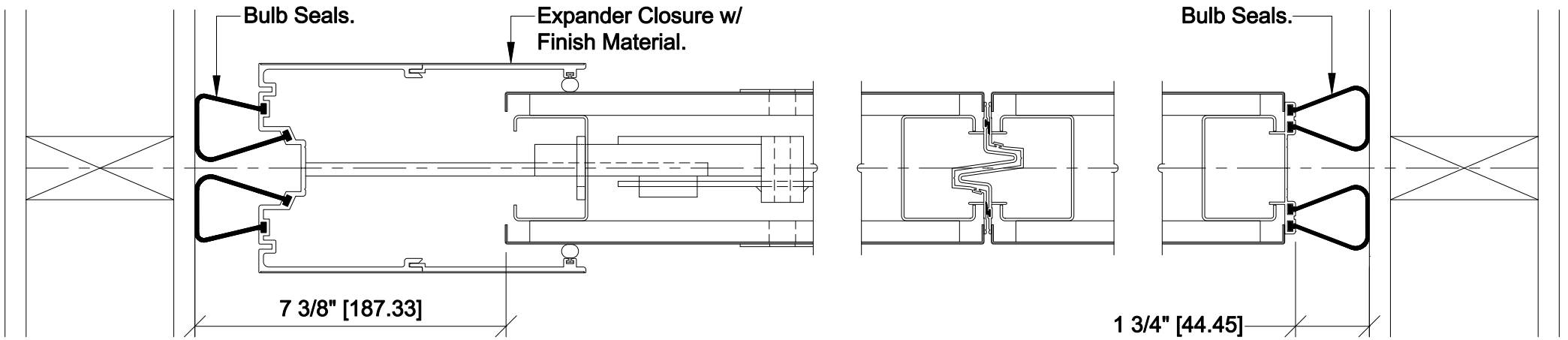
Horizontal Detail - Model 3020 (Trimless)
