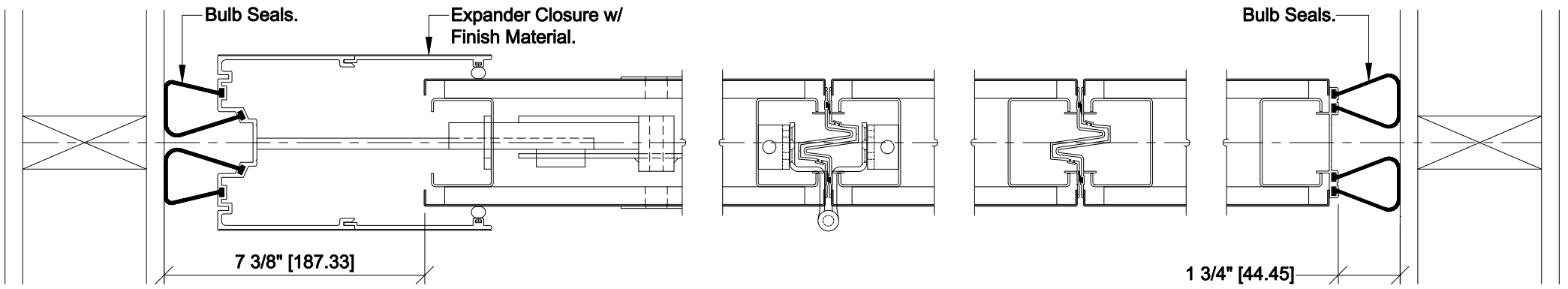
Horizontal Detail - Model 3030 (Trimless)
