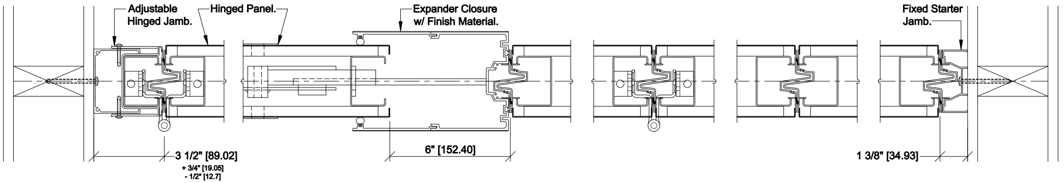
Horizontal Detail - Model 3030 (Trimless)
