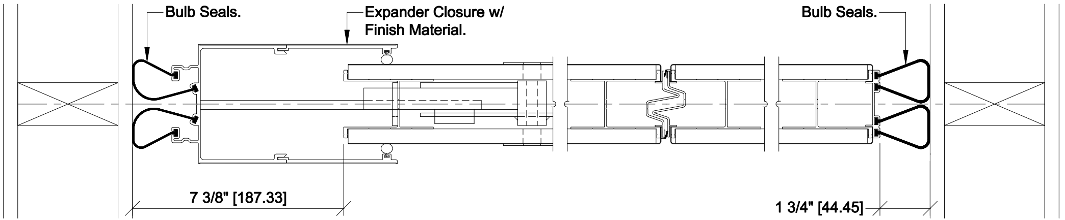
Horizontal Detail - Model 2020 (Trimless)
