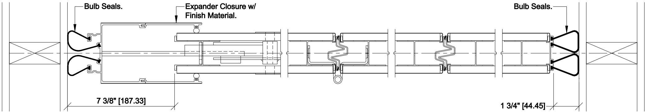
Horizontal Detail - Model 2030 (Trimless)
