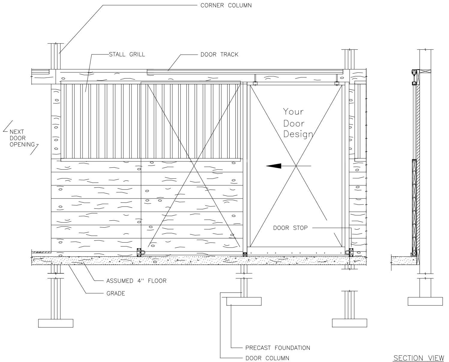
ELEVATION VIEW
