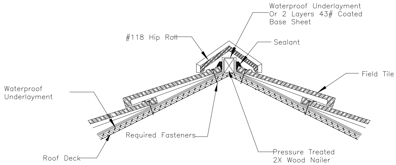
118 HIP DETAIL
