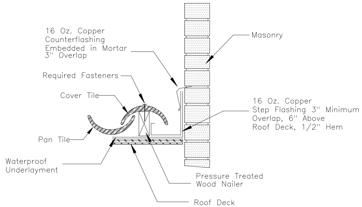
FIG. 9.5 FLASHING AT VERTICAL WALL
