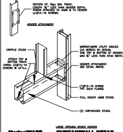
MarinoWARE CURTAINWALL DETAIL
