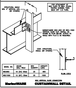
MarinoWARE CURTAINWALL DETAIL
