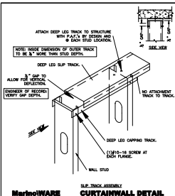
MarinoWARE CURTAINWALL DETAIL
