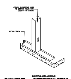
MarinoWARE CURTAINWALL DETAIL
