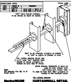
MarinoWARE CURTAINWALL DETAIL
