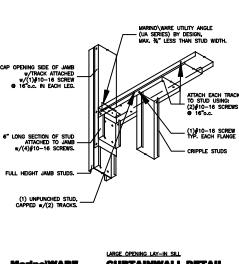
MarinoWARE CURTAINWALL DETAIL
