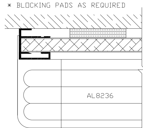
TOP SECTION VIEW SCALE: 1/2
