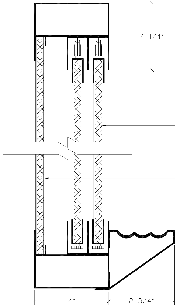
HORIZONTAL SLIDING UNIT
