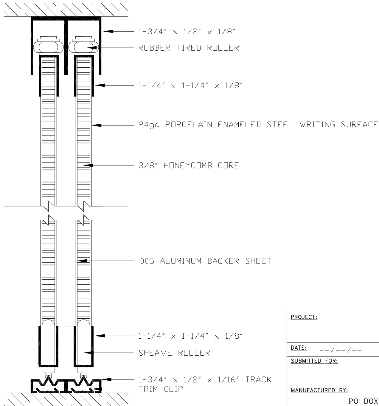
HORIZONTAL SLIDING UNIT RECESSED MOUNTED
