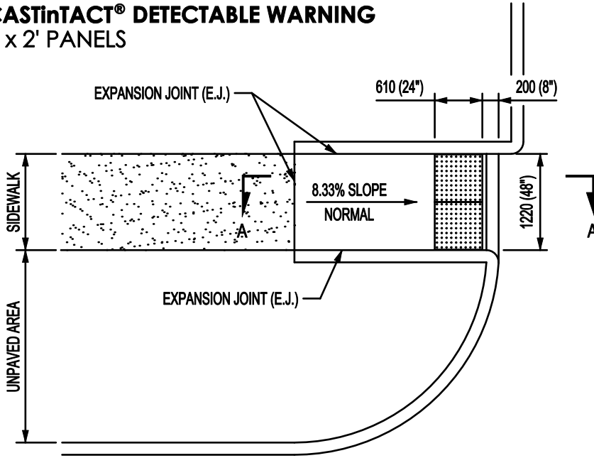
1220mm (48") PARALLEL SIDEWALK RAMP DETAIL OPTION 3
