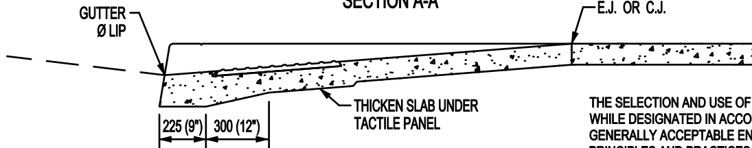
SECTION A-A MONOLITHIC CURB & SIDEWALK
