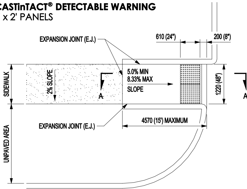
1220mm (48") PARALLEL SIDEWALK RAMP DETAIL OPTION 2
