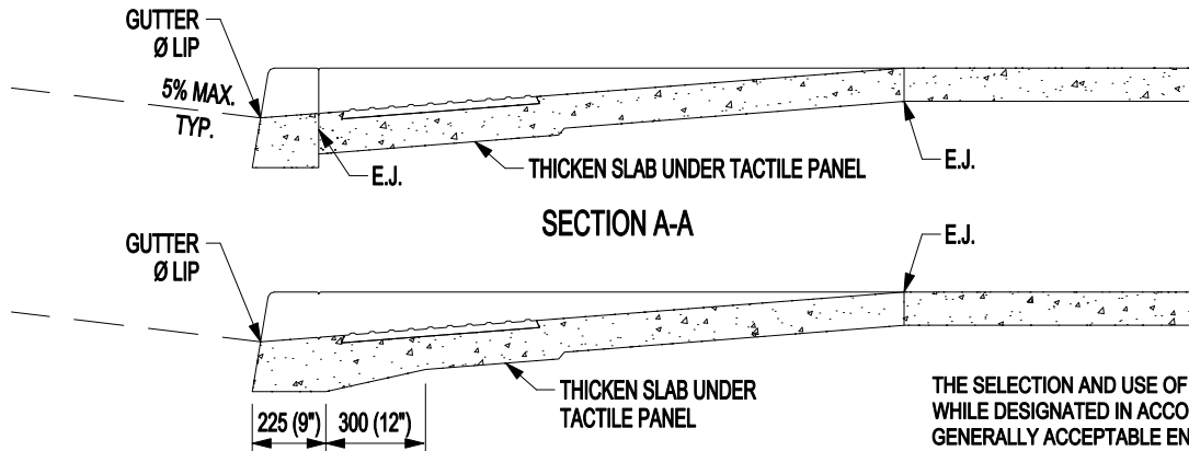
SECTION A-A MONOLITHIC CURB & SIDEWALK
