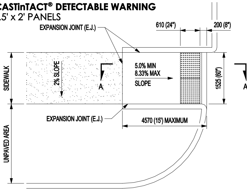
1525mm (60") PARALLEL SIDEWALK RAMP DETAIL OPTION 2
