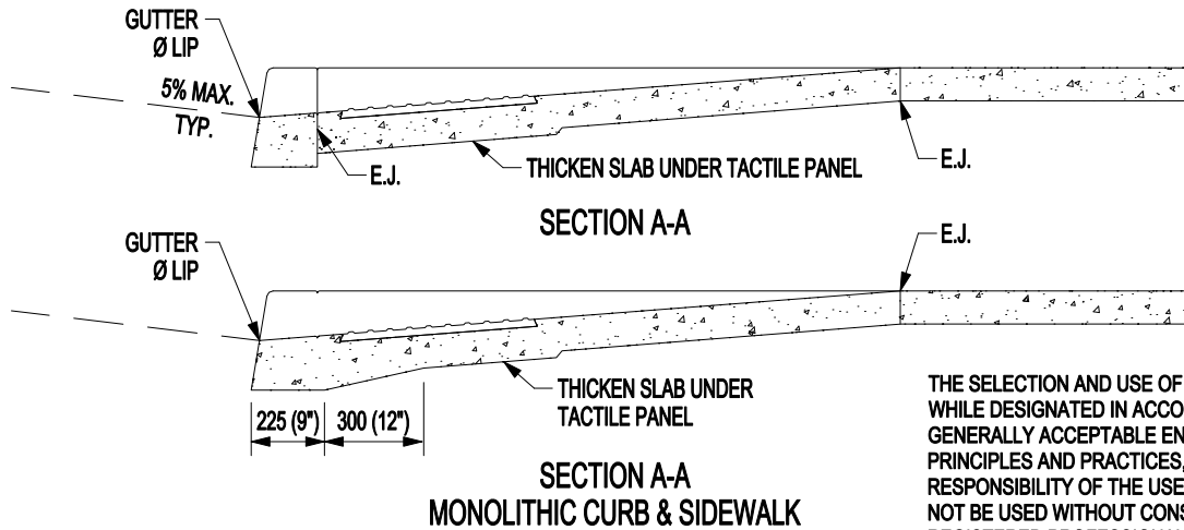
1525mm (60") PARALLEL SIDEWALK RAMP DETAIL OPTION 2
