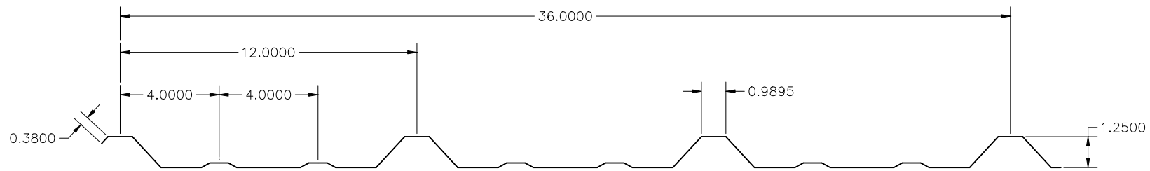
PBR-Panel Profile
