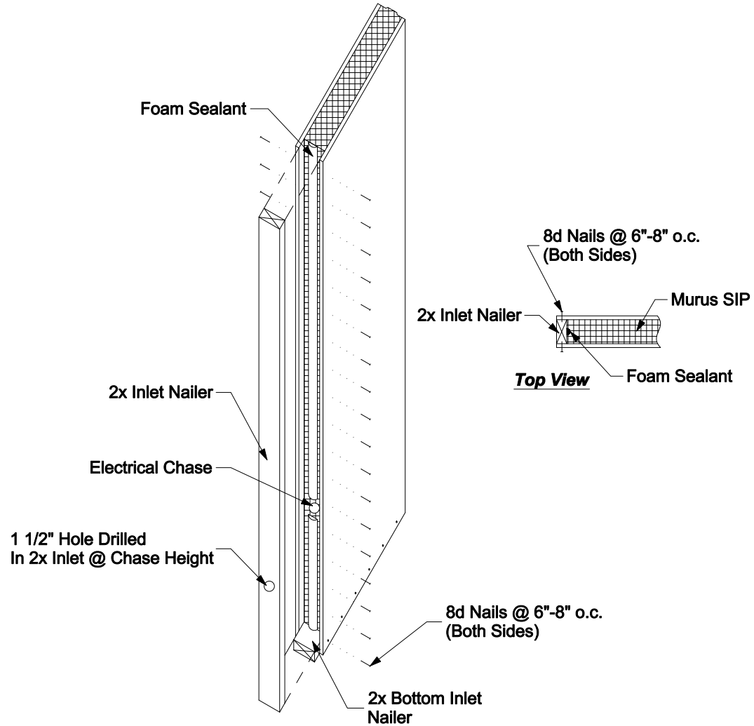
24 3d Inlet Nailer Detail Scale: 3/4" = 1'-0"
