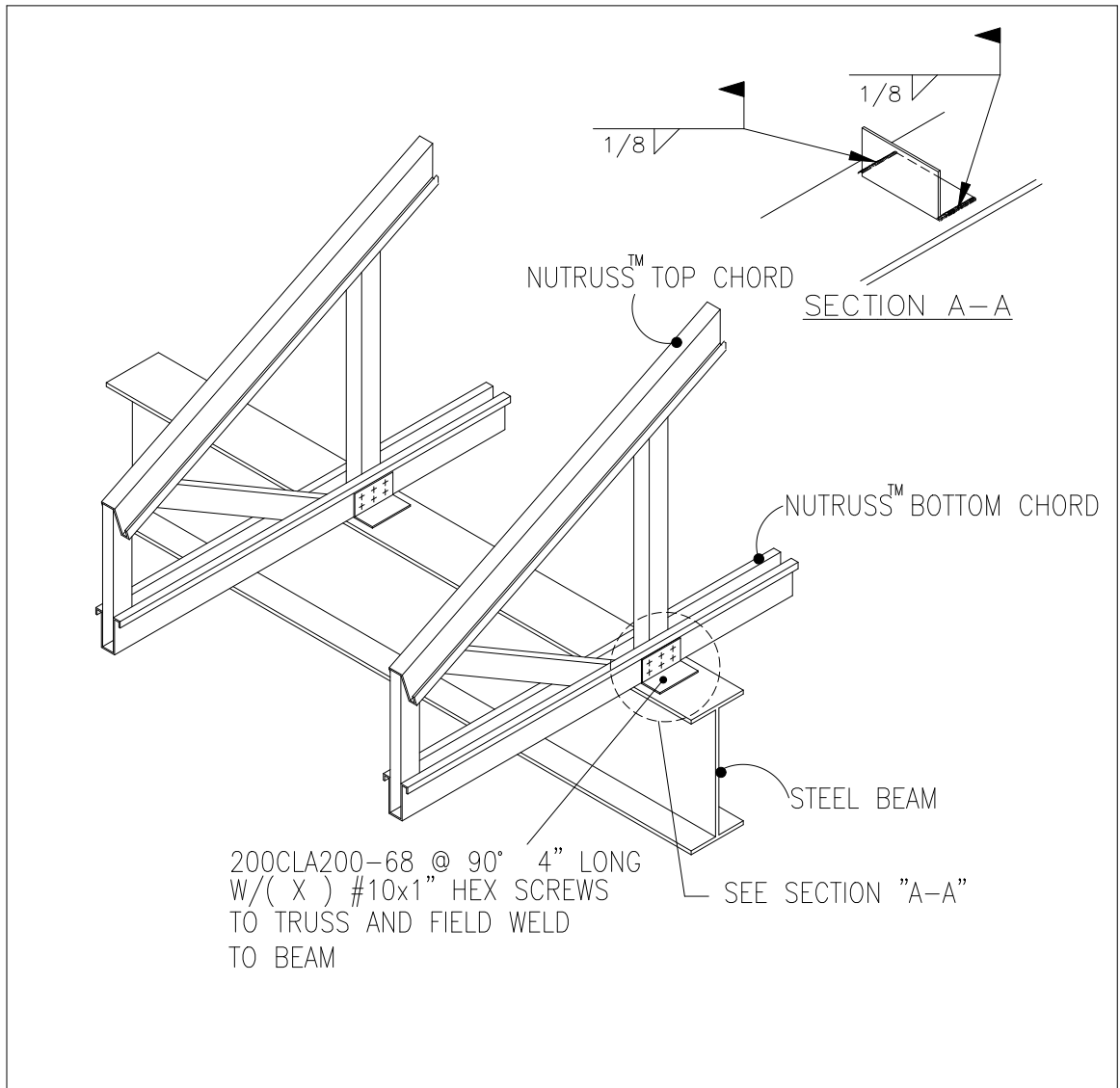
- TRUSS TO BEAM CONNECTION N.T.S. 06-03-03
