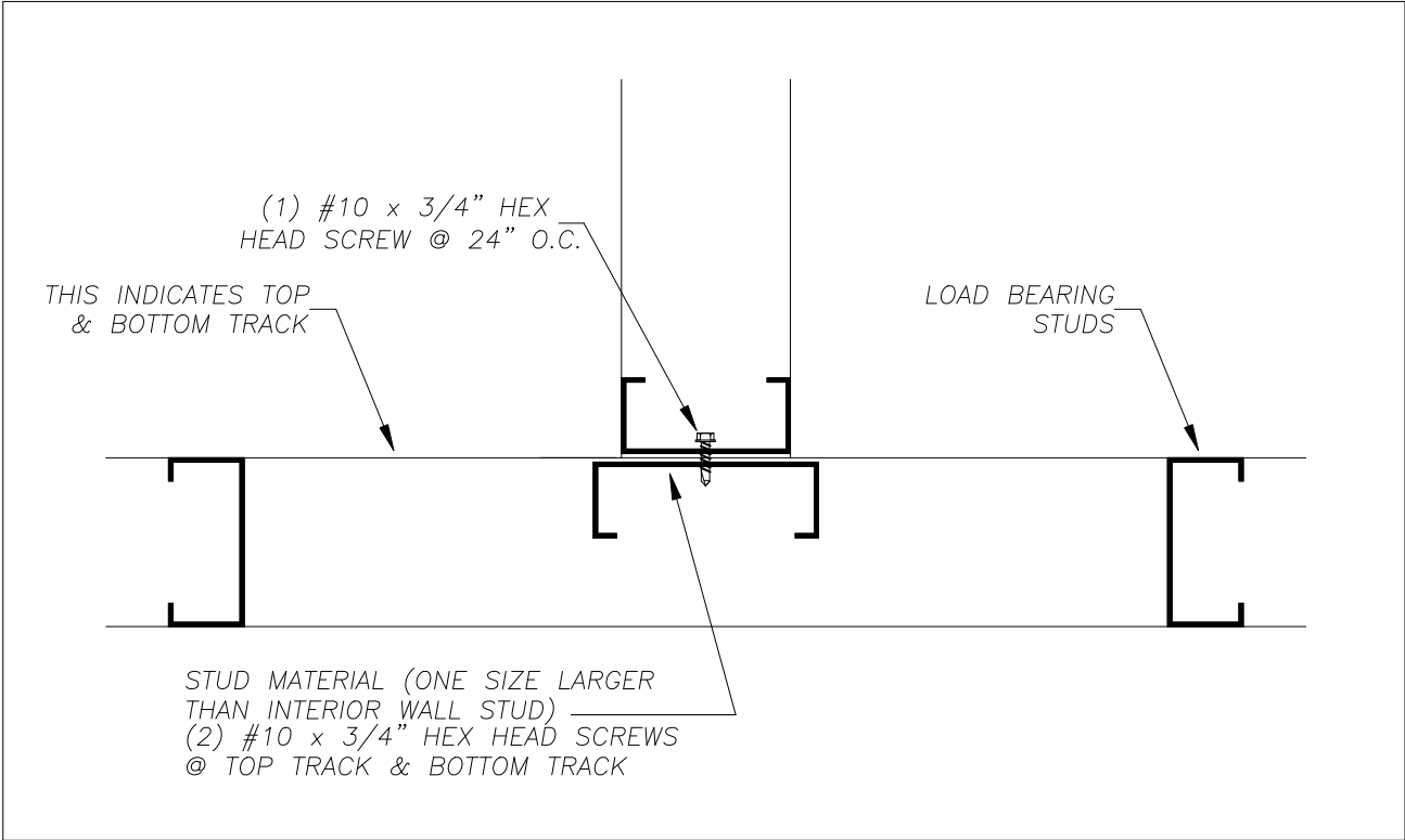
— WALL INTERSECTION FRAMING N.T.S.
