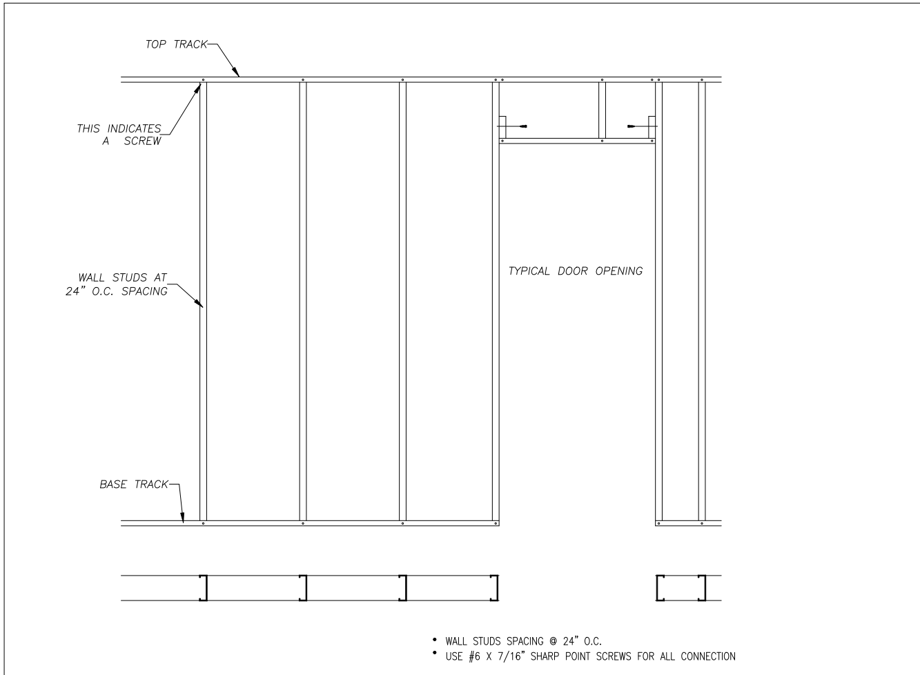
- TYP. NON-STRUCTURAL WALL FRAMING N.T.S. 09/20/02
