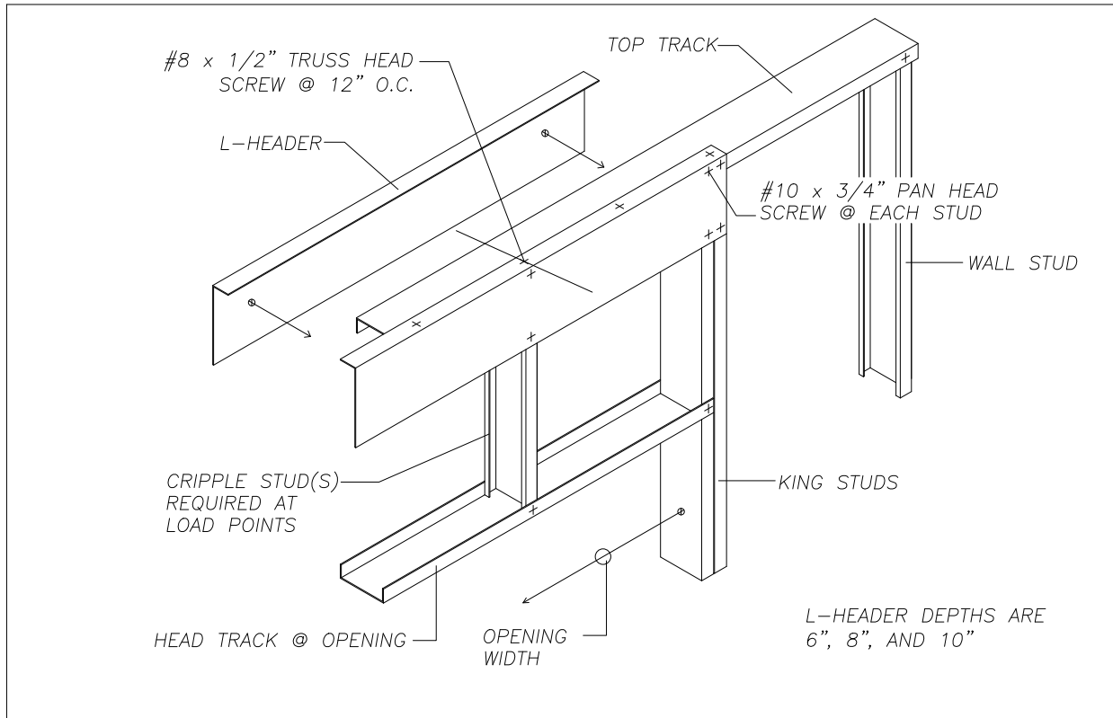
⊖ DOUBLE L-HEADER FRAMING N.T.S. 08-26-03
