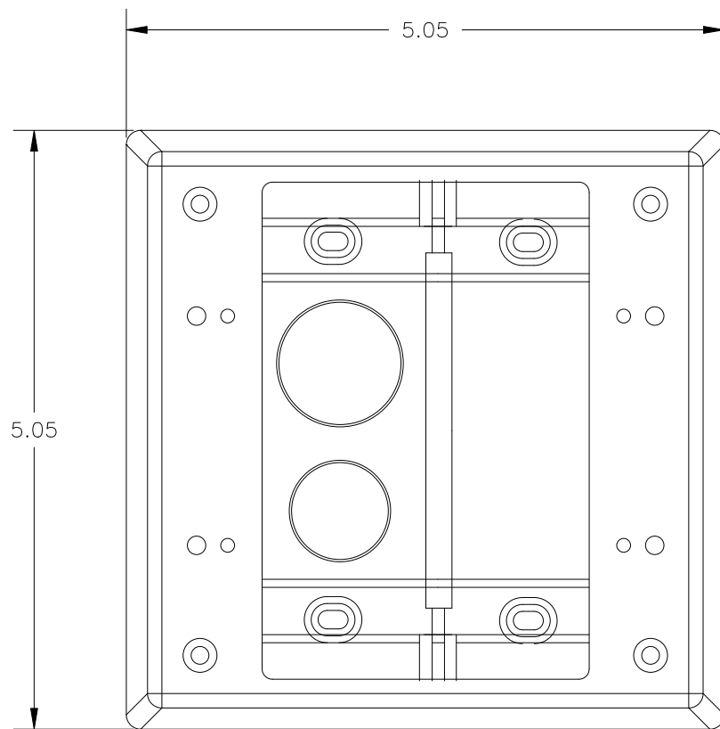
TOP VIEW
