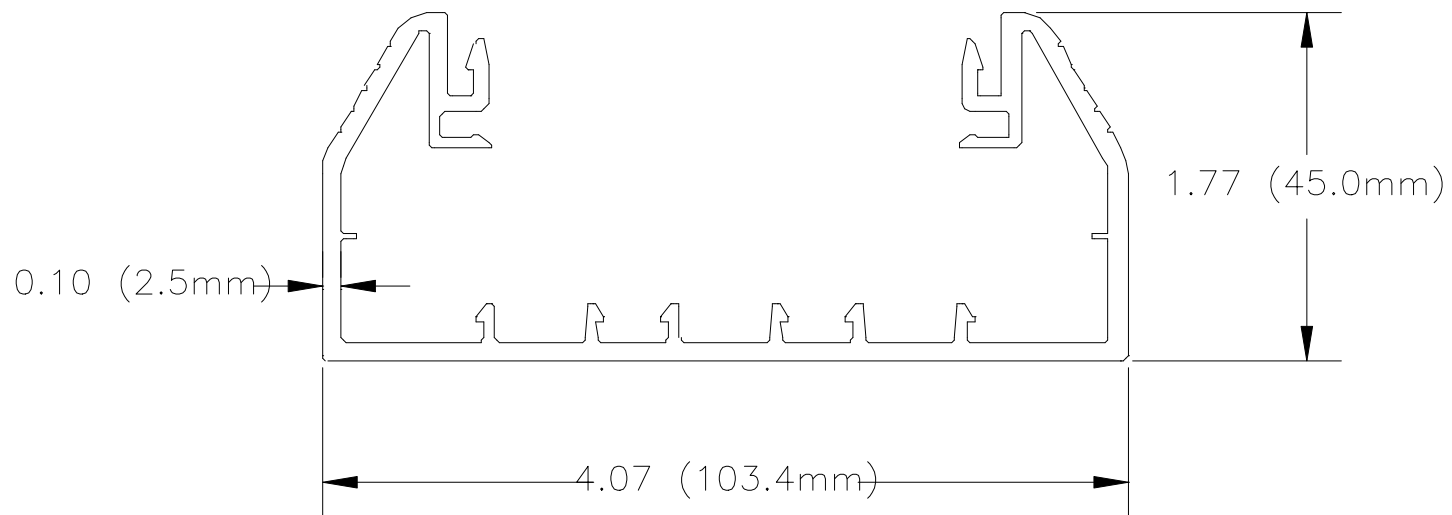
FRONT VIEW
