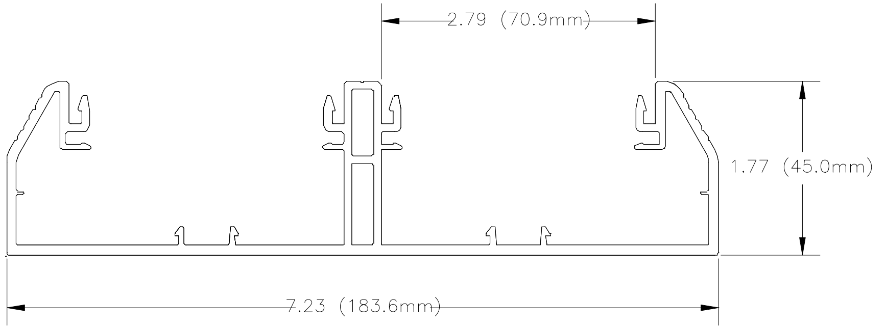
FRONT VIEW
