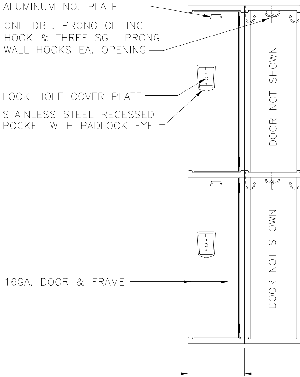
ELEVATION SECTION @ WALL 72" HIGH DOUBLE TIER GUARDIAN KNOCKDOWN LOCKER
