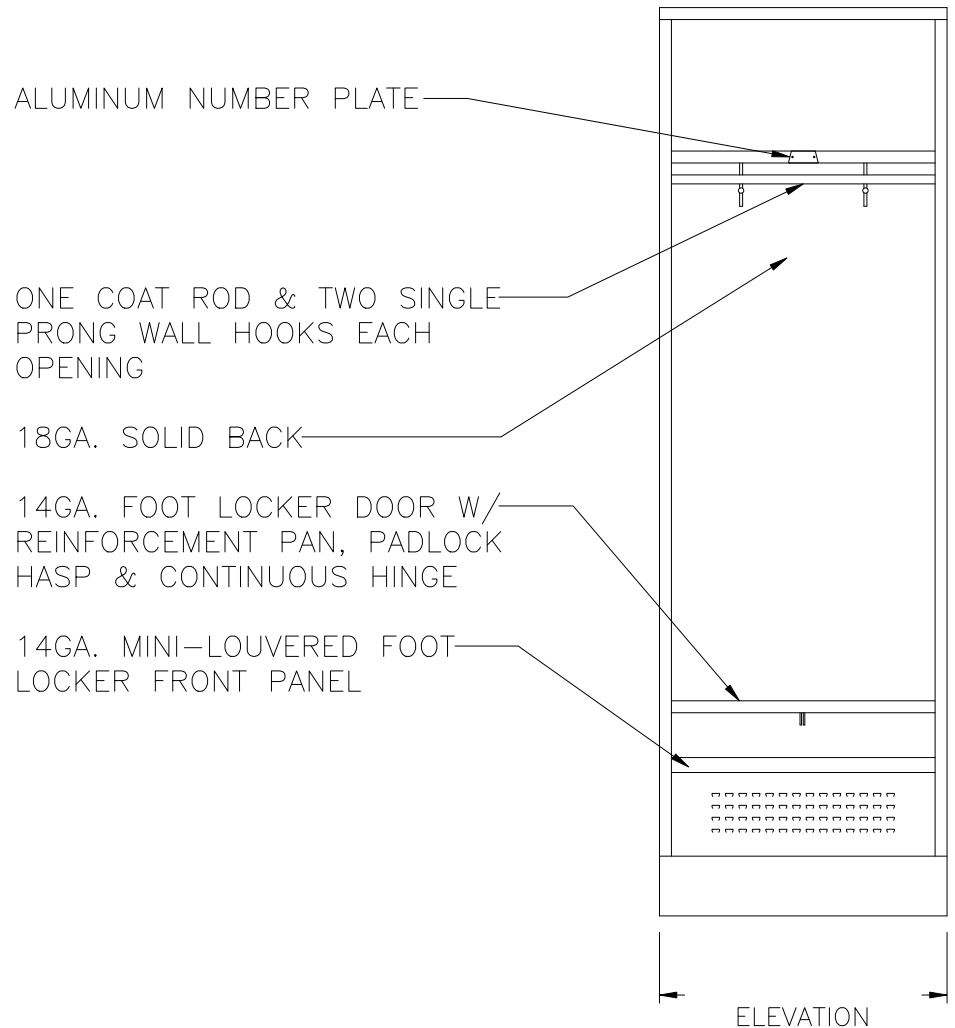
76" STADIUM ALL-WELDED LOCKER W/ SHELF & FOOT LOCKER 24" & 33" WIDE, ALLOW 1/16" CREEPAGE PER FRAME TYPICAL FOR 18", 21" & 24" DEEP
