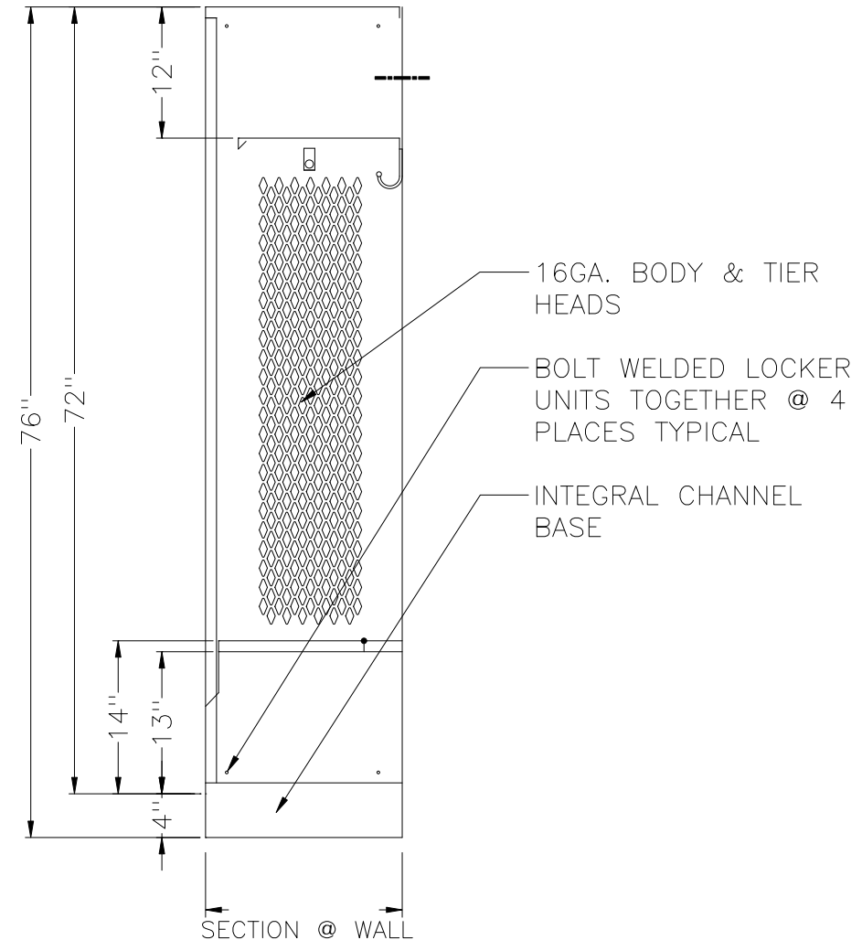
76" STADIUM ALL-WELDED LOCKER W/ SHELF & FOOT LOCKER 24" & 33" WIDE, ALLOW 1/16" CREEPAGE PER FRAME TYPICAL FOR 18", 21" & 24" DEEP
