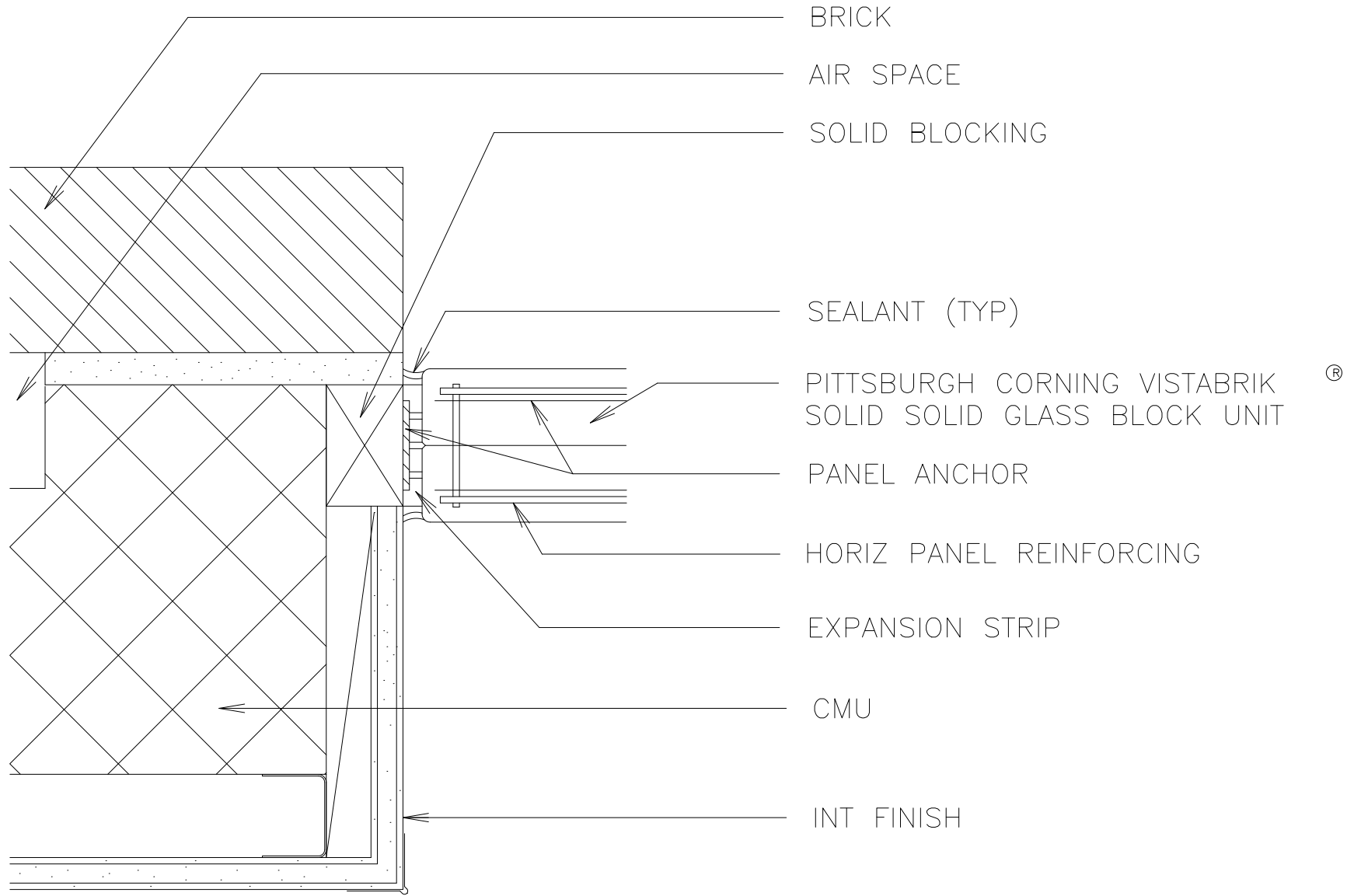
○ JAMB — GLASS BLOCK IN BRICK MASONRY CAVITY WALL
