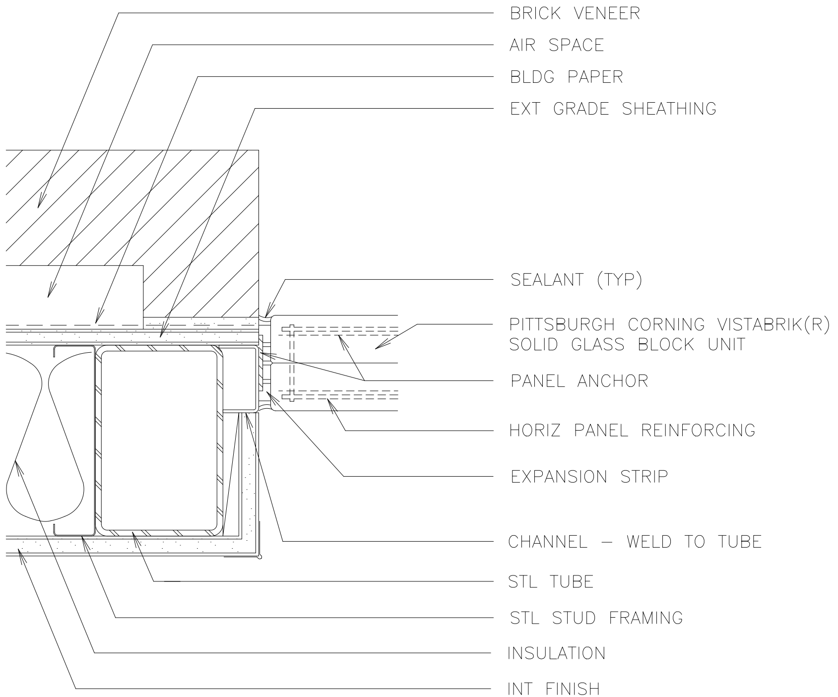
JAMB - GLASS BLOCK IN STEEL STUD WALL WITH BRICK VENEER
