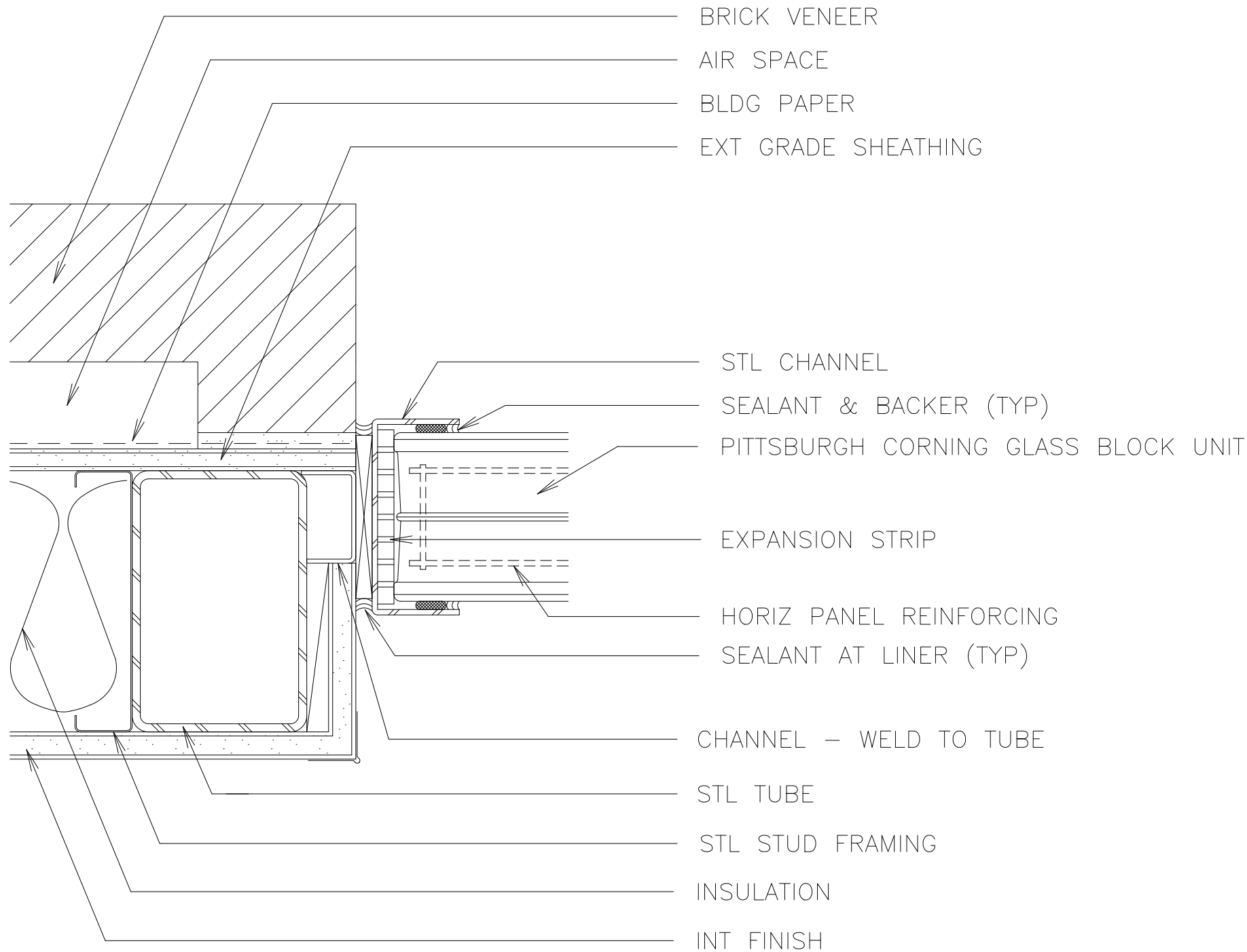
JAMB - GLASS BLOCK IN STEEL STUD WALL WITH BRICK VENEER
