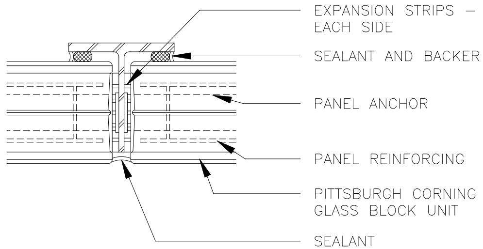
○ ("T" COLUMN) INTERMEDIATE VERTICLE SUPPORT IN MULTIPLE HORIZONTAL PANELS 1/4 FS
