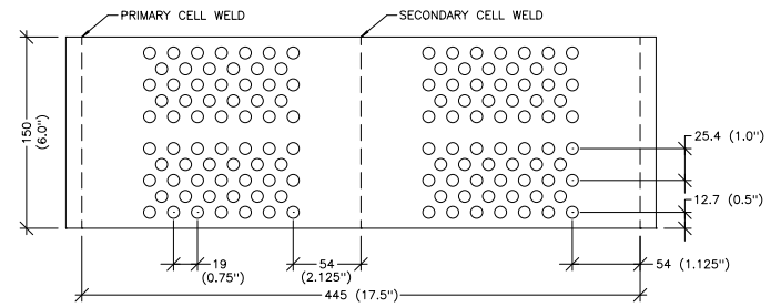
PERFORATION PATTERN - 150 mm (6") COLLAPSED GEOWEB® GW30V SECTIONS
