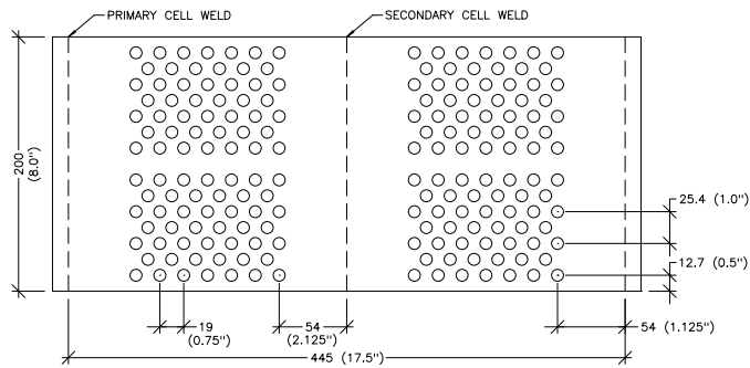
PERFORATION PATTERN - 200 mm (8") COLLAPSED GEOWEB® GW30V SECTIONS
