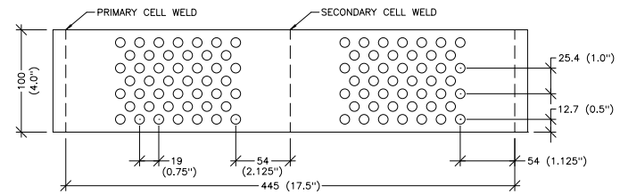
PERFORATION PATTERN - 100 mm (4") COLLAPSED GEOWEB® GW30V SECTIONS
