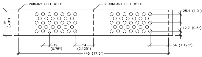
PERFORATION PATTERN - 75 mm (3") COLLAPSED GEOWEB® GW30V SECTIONS
