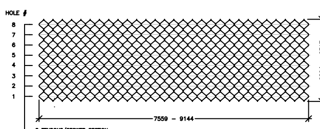
8 TENDON SPACING
