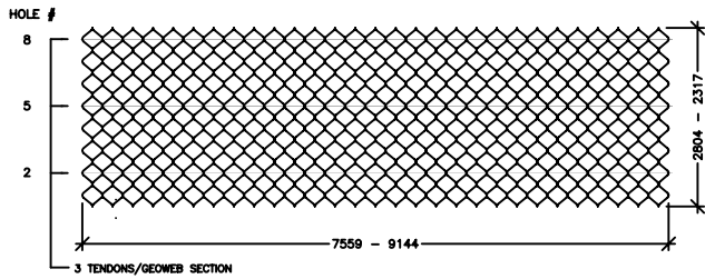
3 TENDON SPACING
