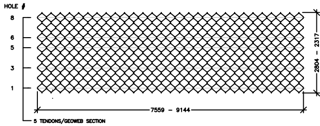
5 TENDON SPACING
