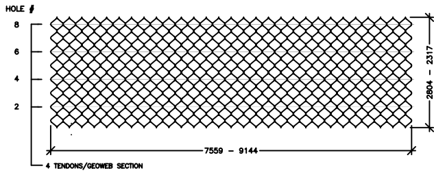
4 TENDON SPACING
