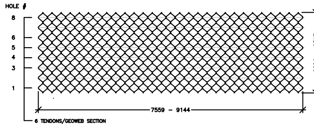
6 TENDON SPACING
