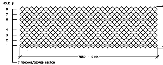
7 TENDON SPACING
