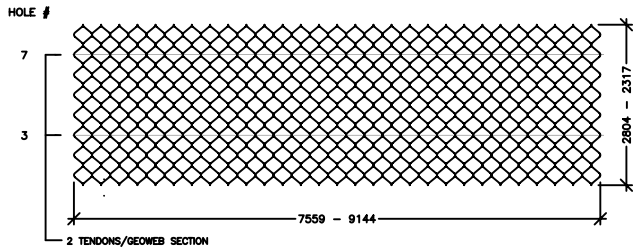
2 TENDON SPACING
