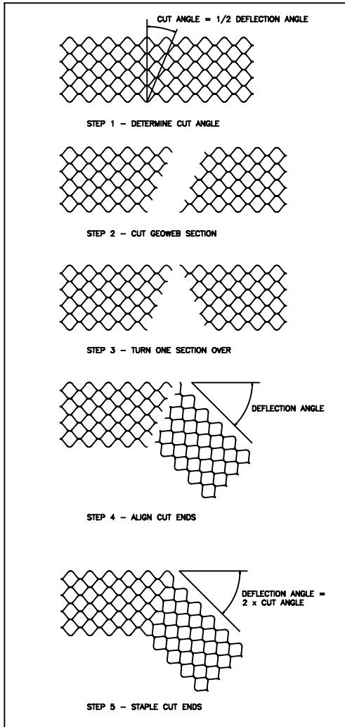
GEOWEB® WALL BEND CUT DETAILS STANDARD COLOR FACE - MINIMUM WASTAGE
