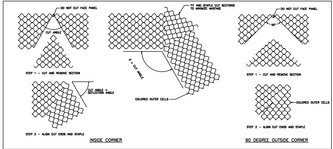
GEOWEB® WALL BEND CUT DETAILS - COLORED FRONT FACE
