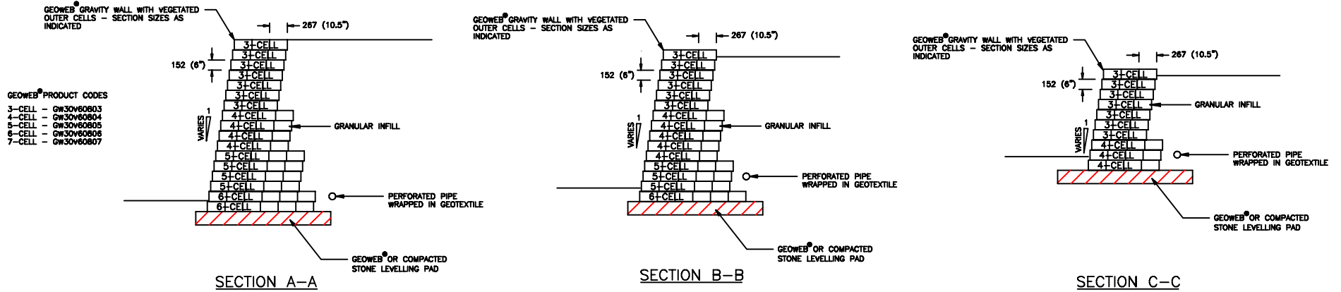
CROSS SECTIONS OF TYPICAL GEOWEB® GRAVITY WALL
