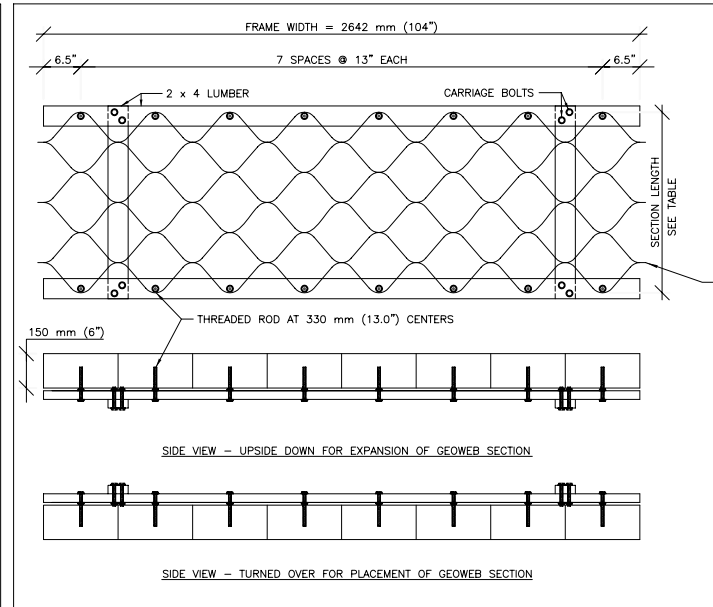
TYPICAL WOOD STRETCHER FRAME FOR GW30V60803 SECTION SIZE
