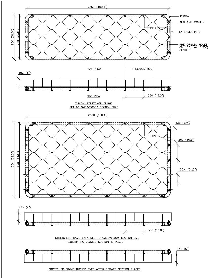
EXPANDABLE STRETCHER FRAME WITH EXTENDER PIPES FOR GW30V60803 TO GW30V60806 SECTIONS
