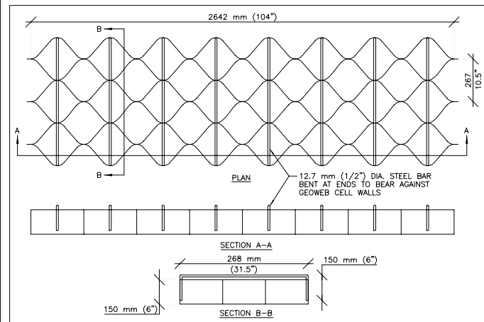
TEMPORARY STRETCHING METHOD FOR INSTALLATION OF GW30V GEOWEB SECTIONS
