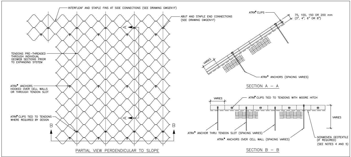
TYPICAL ATRA® CLIP, TENDON AND ATRA® ANCHOR SYSTEM
