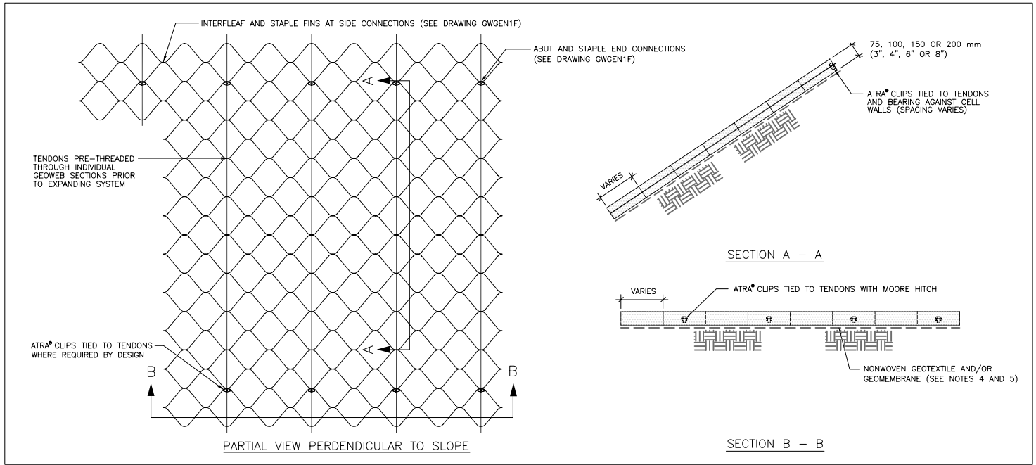
TYPICAL ATRA® CLIP AND TENDON SYSTEM
