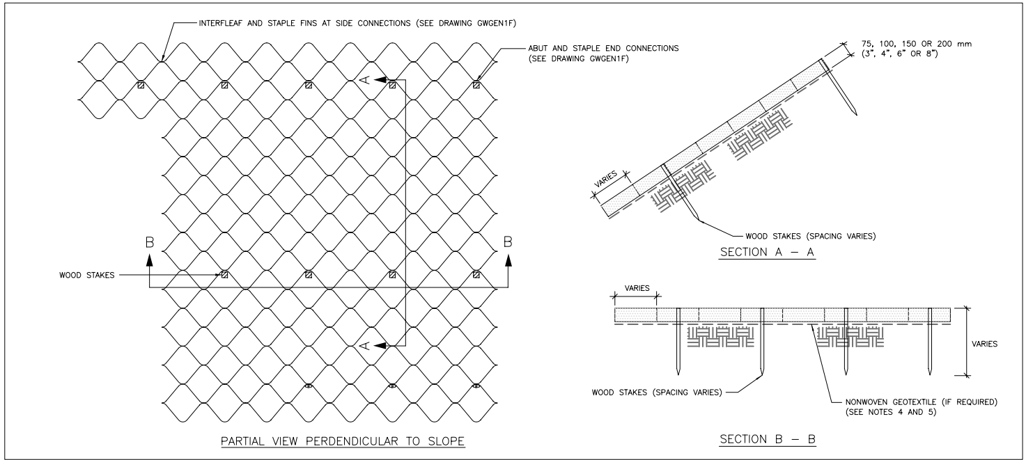
TYPICAL WOOD STAKE TEMPORARY ANCHOR SYSTEM
