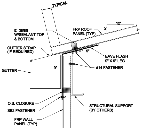
EAVE DETAIL W/GUTTER
