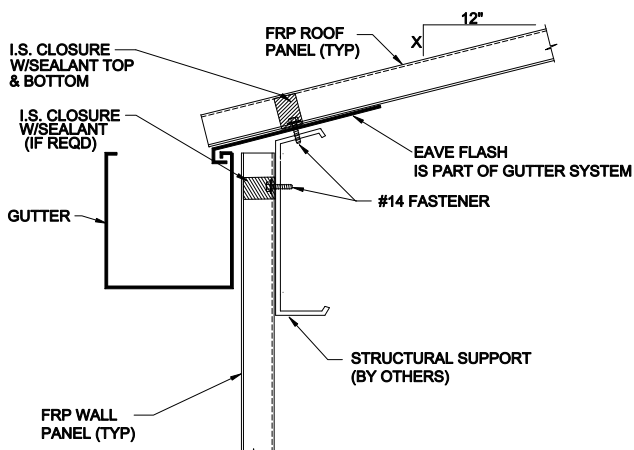
EAVE DETAIL (WITH FRP GUTTER)
