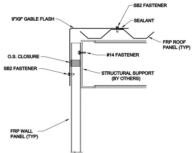
GABLE DETAIL
