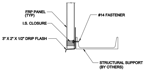
HEAD DETAIL (STANDARD FLASH)
