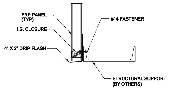
HEAD DETAIL (NONSTANDARD FLASH)
