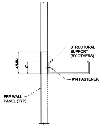
SIDING END LAP DETAIL
