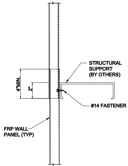
SIDING END LAP DETAIL
