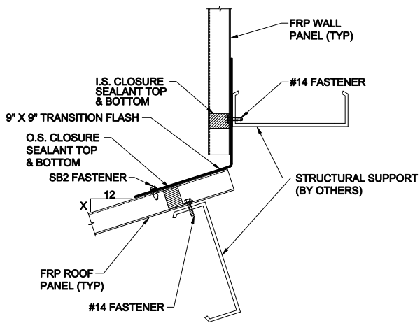
TRANSITION (HEADWALL) DETAIL
