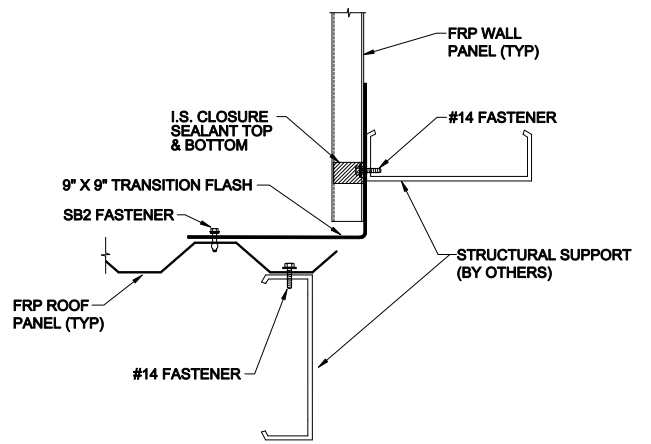
TRANSITION (SIDE WALL) DETAIL
