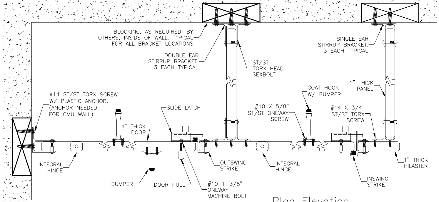
Plan Elevation
