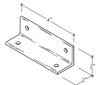
"L" BRACKET N T S
