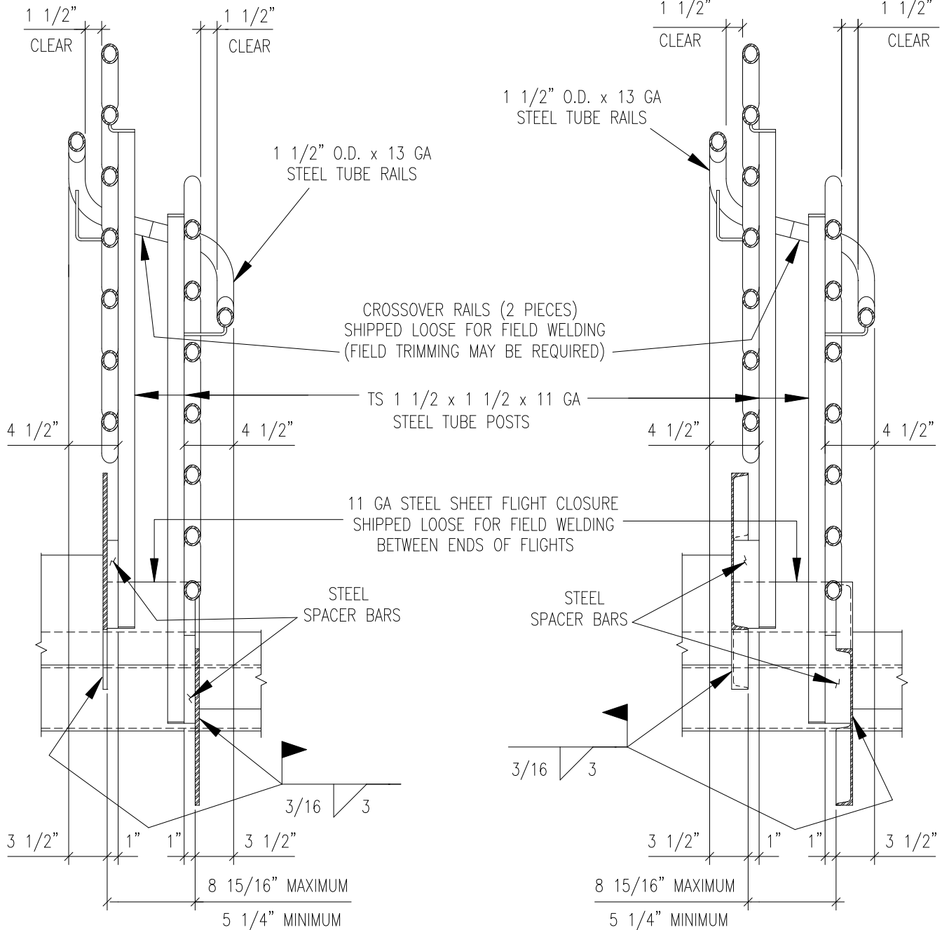
SECTION C PLATE STRINGERS
