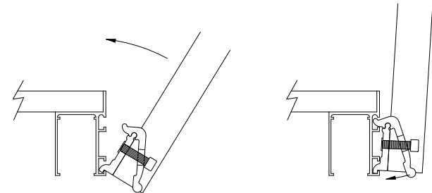
ATTACHMENT DETAIL
