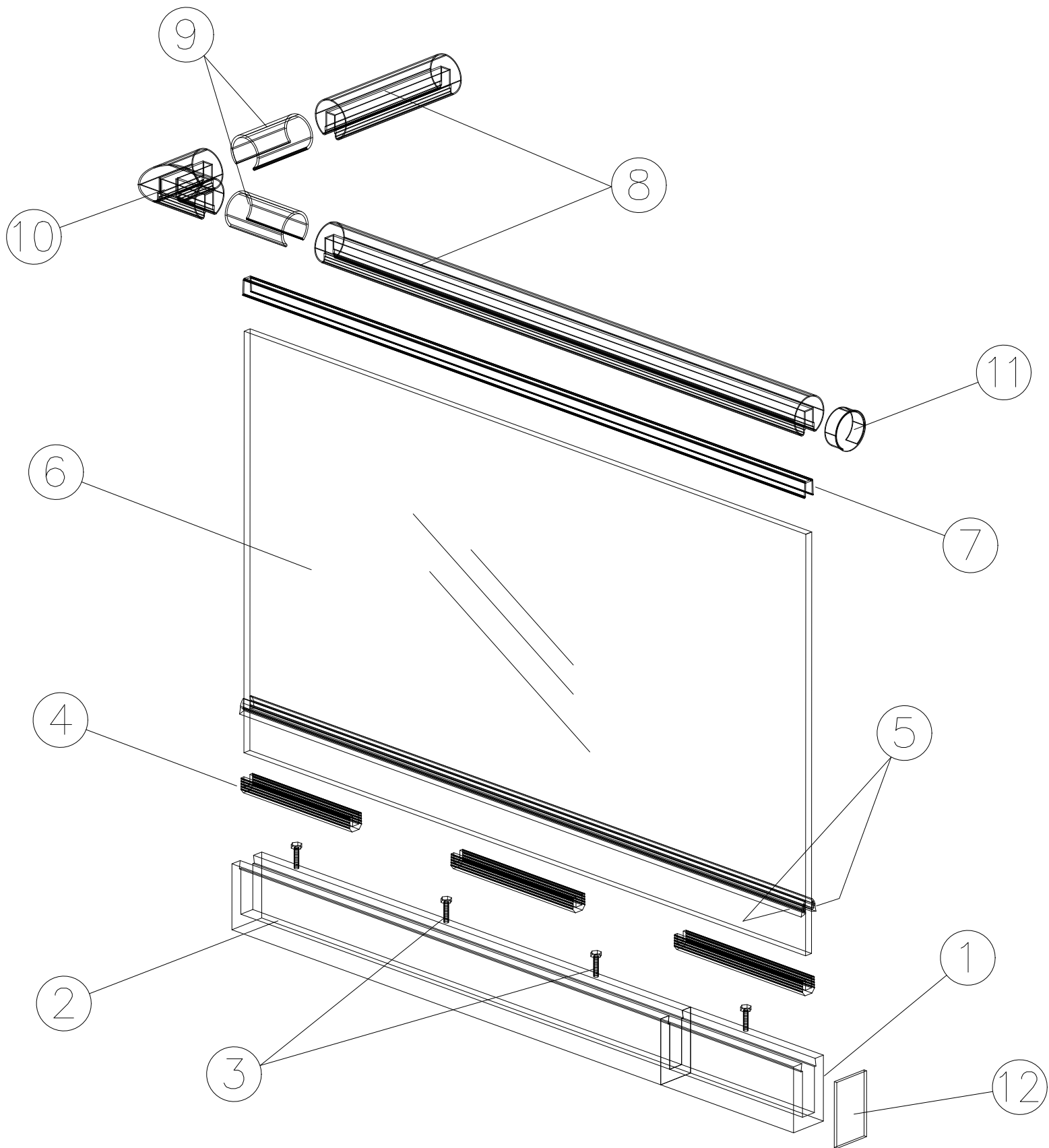
EXPLODED VIEW SCALE: 2" = 1'
