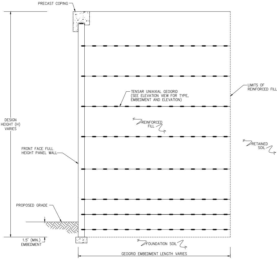
TYPICAL CROSS-SECTION-FULL HEIGHT PANEL WALL
