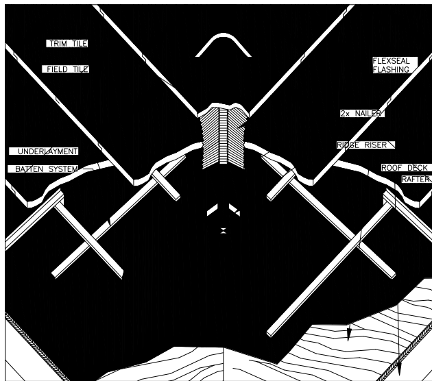
HIP ROOF APPLICATION - FLAT TILE
