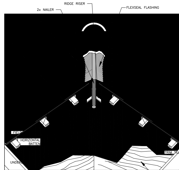
HIP ROOF APPLICATION: S-TILE
