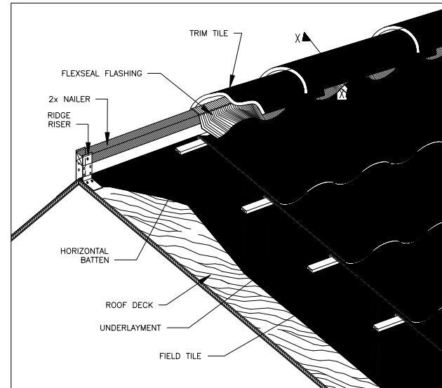
RIDGE APPLICATION: S-TILE
